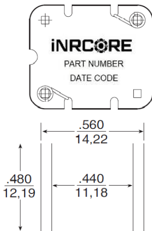
SUGGESTED PAD LAYOUT
