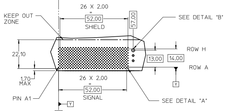
CIRCUIT BOARD HOLE PATTERN (CONNECTOR SIDE)
