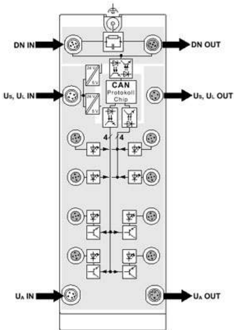
Block diagram
