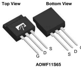
TO-262F
