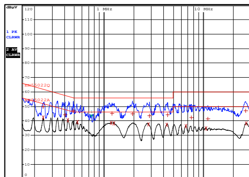
Conducted EMI Neutral Wire
