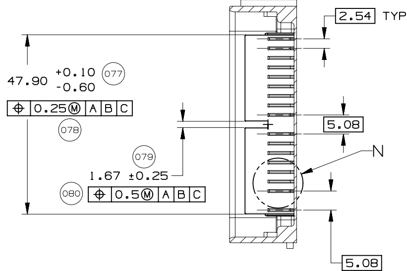
SECTION J-J
