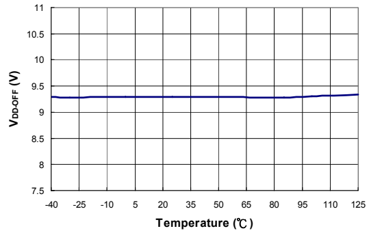
Figure 12. Minimum Operating Voltage ( V_{DD-OFF} ) vs. Temperature
