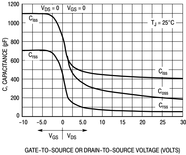
Figure 7. Capacitance Variation
