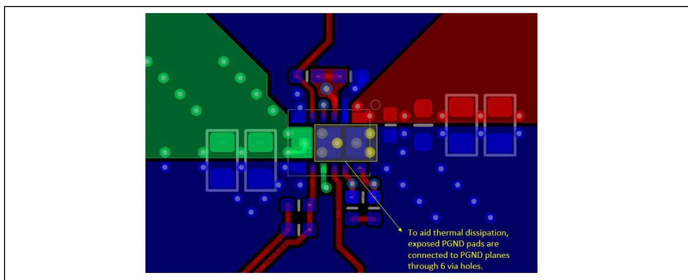
Figure 35 Demo Board Layout – PGND pads
