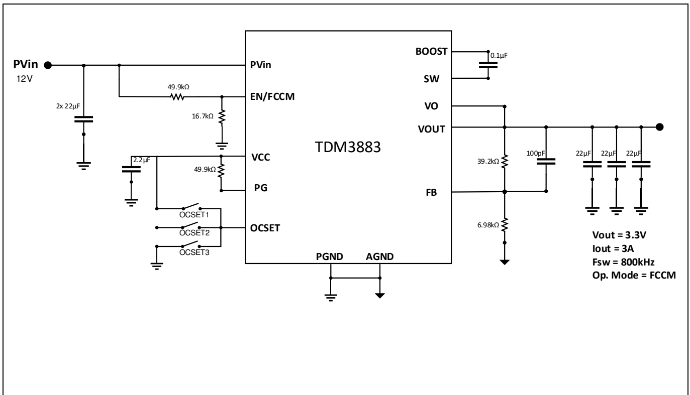
Figure 19 Application Diagram V_{in} = 12\text{ V} , V_{out} = 3.3\text{ V} , I_{out} = 3\text{ A} , FCCM
