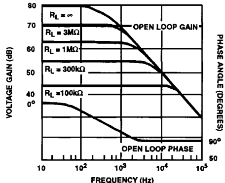
FIGURE 6. OPEN-LOOP AMPLIFIER RESPONSE CHARACTERISTICS.
