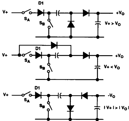
FIGURE 15. CAPACITOR-DIODE COUPLED VOLTAGE MULTIPLIER OUTPUT STAGES
