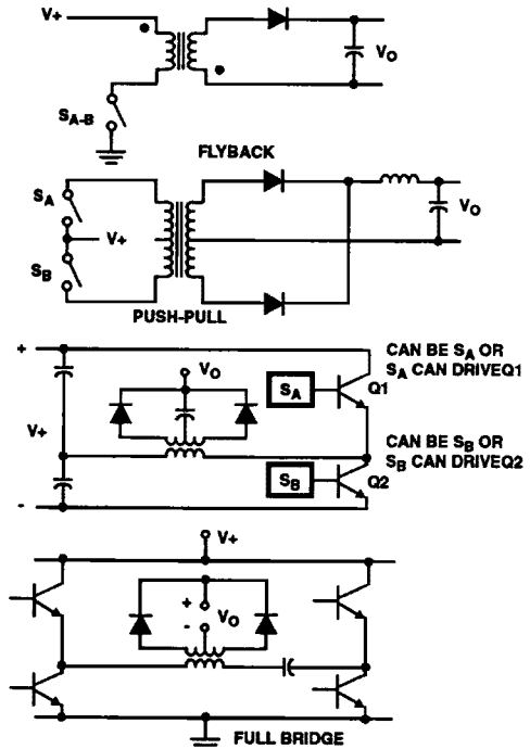
FIGURE 17. TRANSFORMER-COUPLED OUTPUTS
