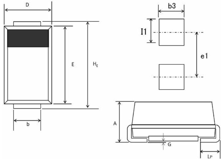
DO-214AC(SMA), (FMDS)
