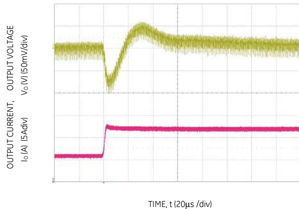
Figure 28. Transient Response to Dynamic Load Change from 50% to 100% at 12V in , C out = 2x47µF+1x330µF, C Tune =2700pF & R Tune =300Ω
