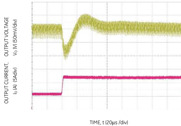
Figure 34. Transient Response to Dynamic Load Change from 50% to 100% at 12Vin, C_{out} = 1 \times 47\mu F + 1 \times 330\mu F , C_{Tune}=2200pF & R_{Tune}=300\Omega
