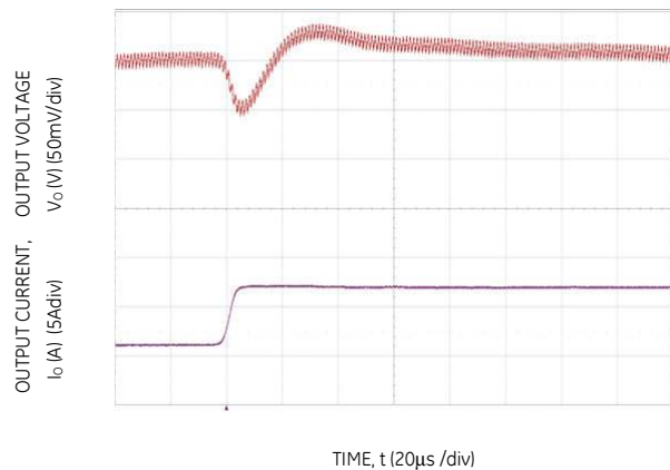
Figure 22. Transient Response to Dynamic Load Change from 50% to 100% at 12Vin, C_{out} = 2 \times 47 \mu F + 1 \times 330 \mu F , C_{Tune} = 3300 pF & R_{Tune} = 240 \Omega
