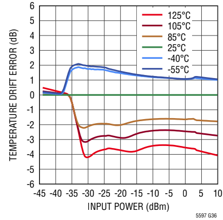
Linearity Error Temperature Variation from 25°C at 70GHz
