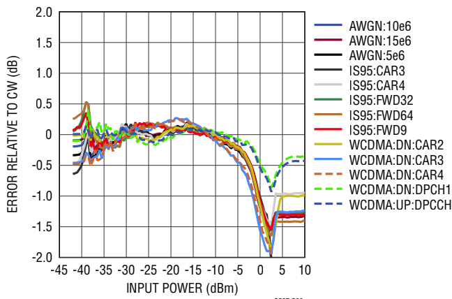
Power Measurement Error Relative to CW for Various Modulation Formats
