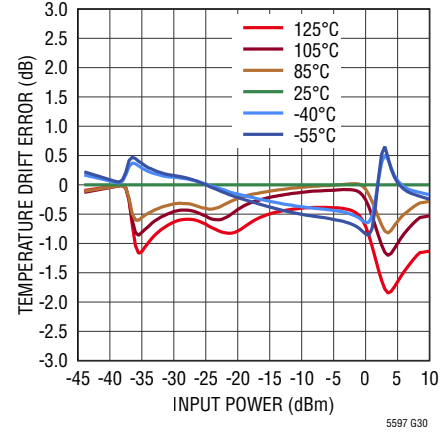
Linearity Error Temperature Variation from 25°C at 39GHz
