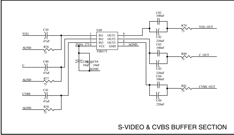
Figure 6. STEVAL-CCH002V2 circuit schematics (6 of 6)
