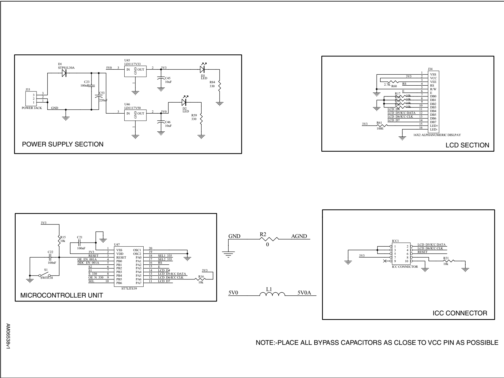
Figure 3. STEVAL-CCH002V2 circuit schematics (3 of 6)
