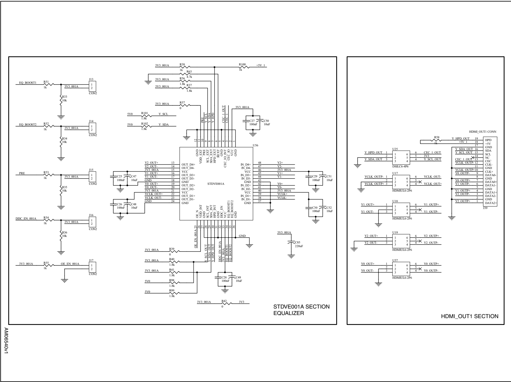
Figure 5. STEVAL-CCH002V2 circuit schematics (5 of 6)
