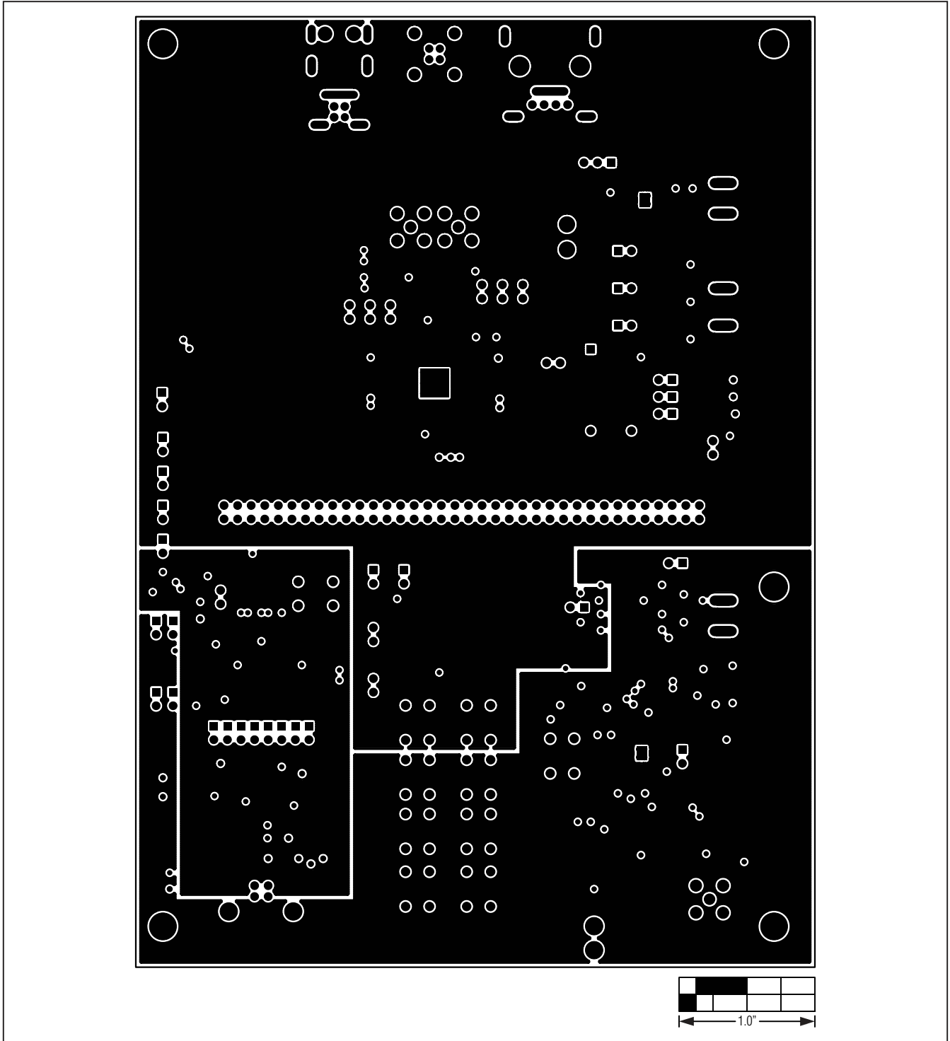
Figure 12. MAX9259 EV Kit PCB Layout—Power Layer 3
