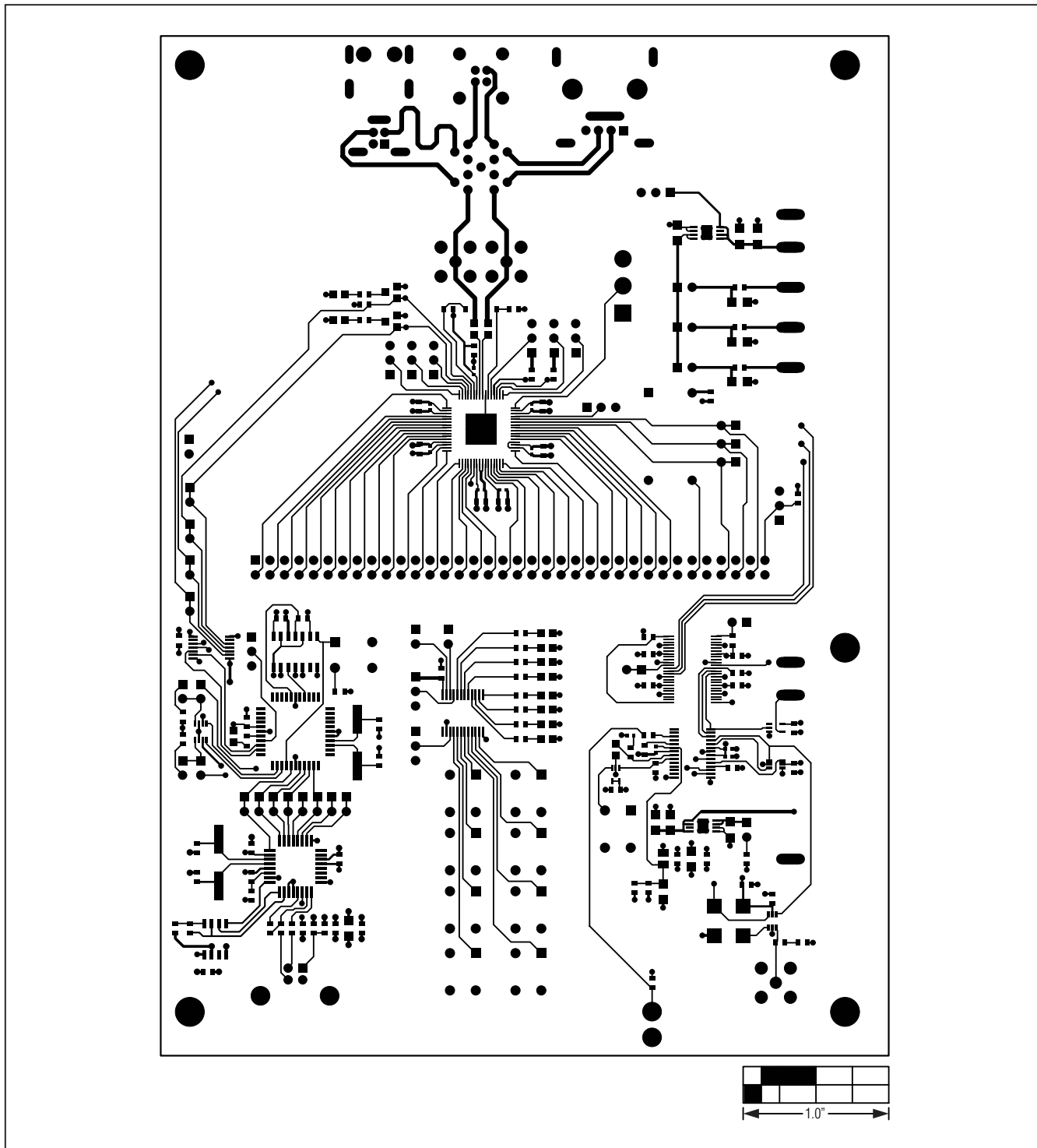
Figure 10. MAX9259 EV Kit PCB Layout—Component Side
