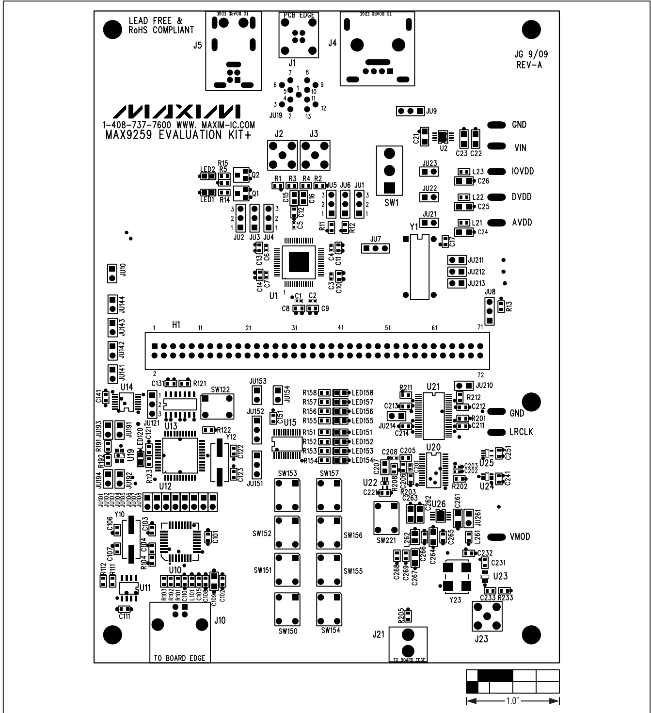
Figure 9. MAX9259 EV Kit Component Placement Guide—Component Side
