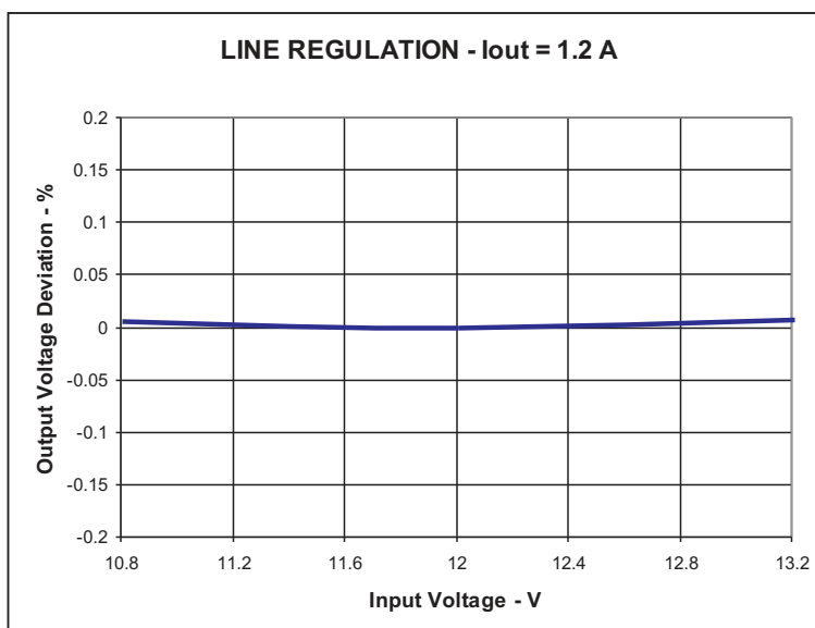
Figure 4. TPS54260EVM-597 Line Regulation
