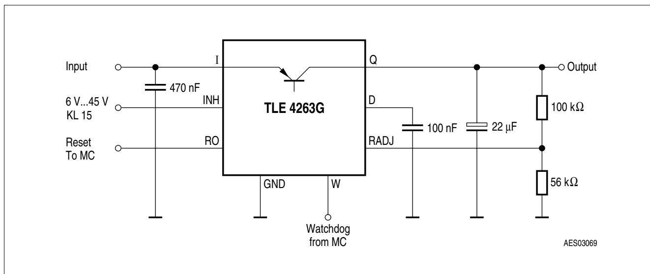
Figure 3 Application circuit
