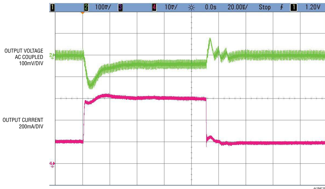
V_{IN} = 12V, V_{OUT1} = 1.5V, 400mA Load Step (200mA <-> 600mA) Pulse-Skipping Mode, f_{SW} = 2.25MHz
