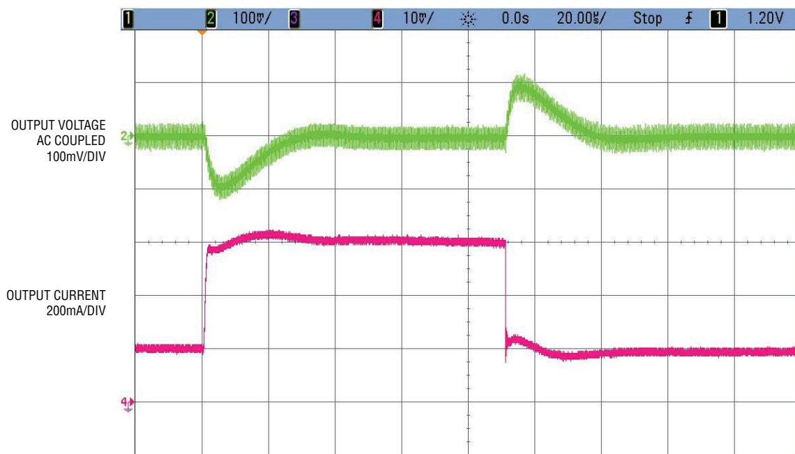
V_{IN} = 12V, V_{OUT1} = 1.8V, 400mA Load Step (200mA <-> 600mA) Pulse-Skipping Mode, f_{SW} = 2.25MHz
