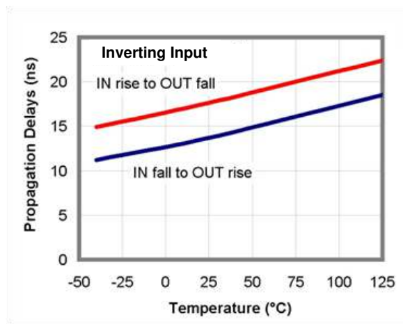
Figure 18. Propagation Delay vs. Temperature
