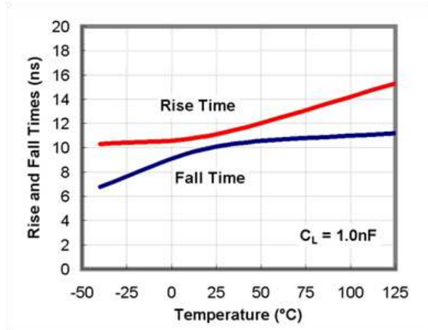
Figure 21. Rise and Fall Time vs. Temperature
