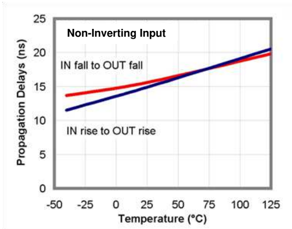
Figure 17. Propagation Delay vs. Temperature
