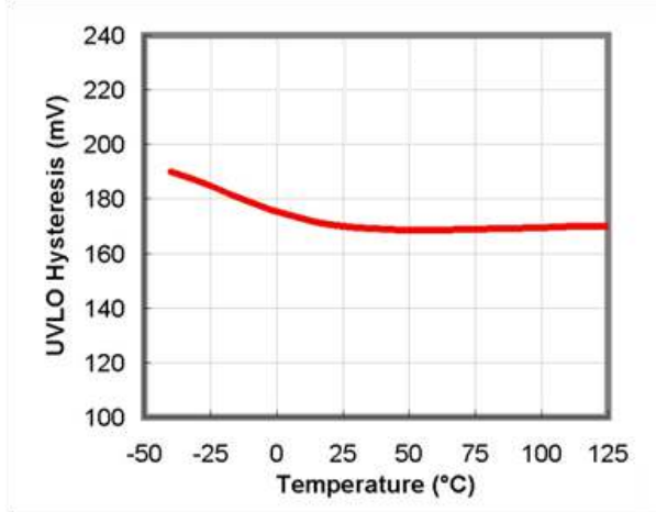
Figure 15. UVLO Hysteresis vs. Temperature
