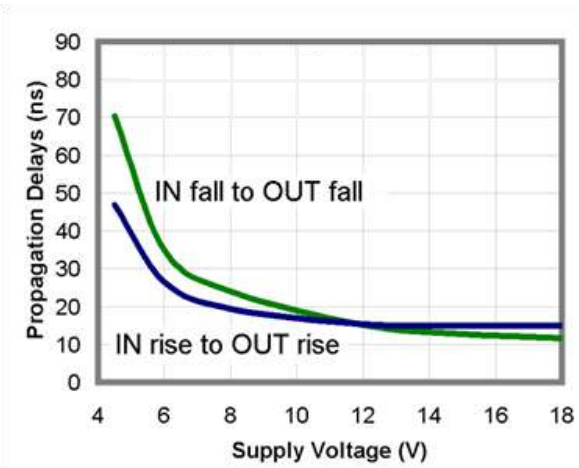
Figure 16. Propagation Delay vs. Supply Voltage
