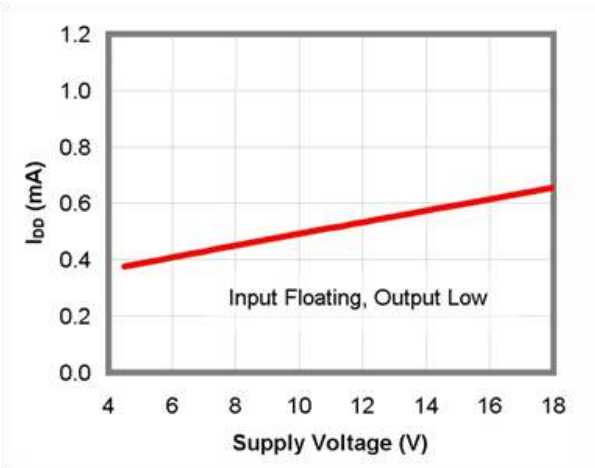
Figure 8. I_{DD} (Static) vs. Supply Voltage
