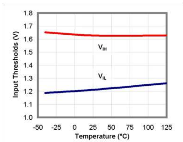
Figure 13. TTL Input Thresholds vs. Temperature
