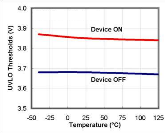
Figure 14. UVLO Thresholds vs. Temperature
