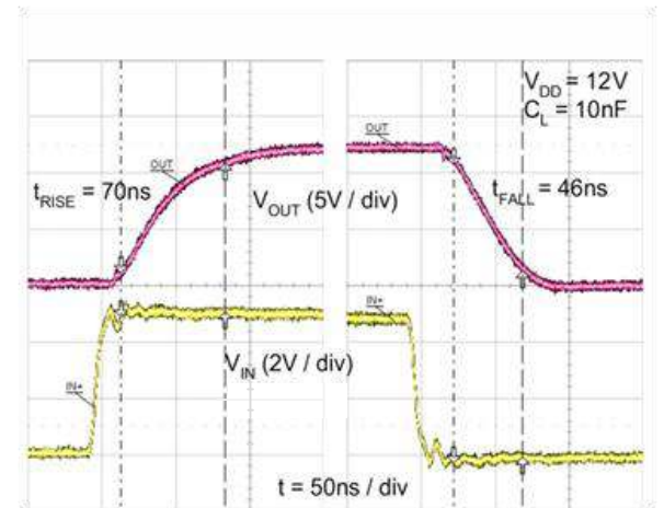
Figure 23. Rise / Fall Waveforms with 10 nF Load
