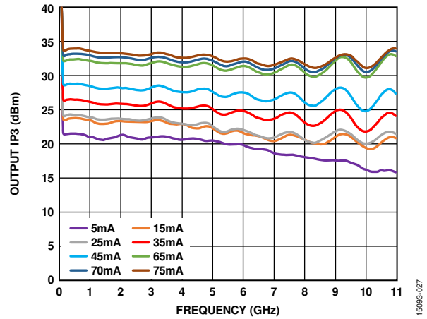
Figure 27. Output IP3 vs. Frequency for Various Supply Currents ( I_{DQ} ), P_{OUT}/Tone = 5 dBm , V_{DD} = 5 V
