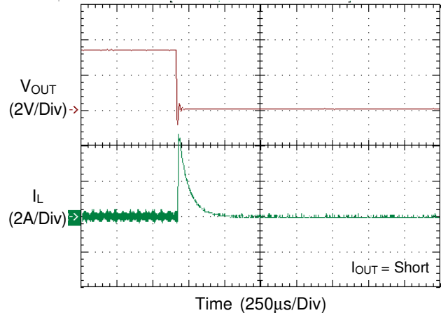
Figure 6. Latch-Off Mode Under Voltage Protection
