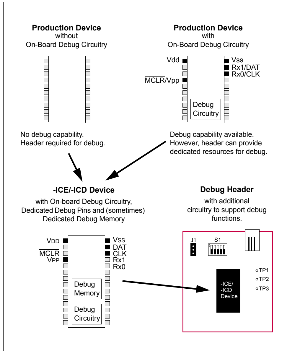
FIGURE 1-2: DEBUG OPTIONS
