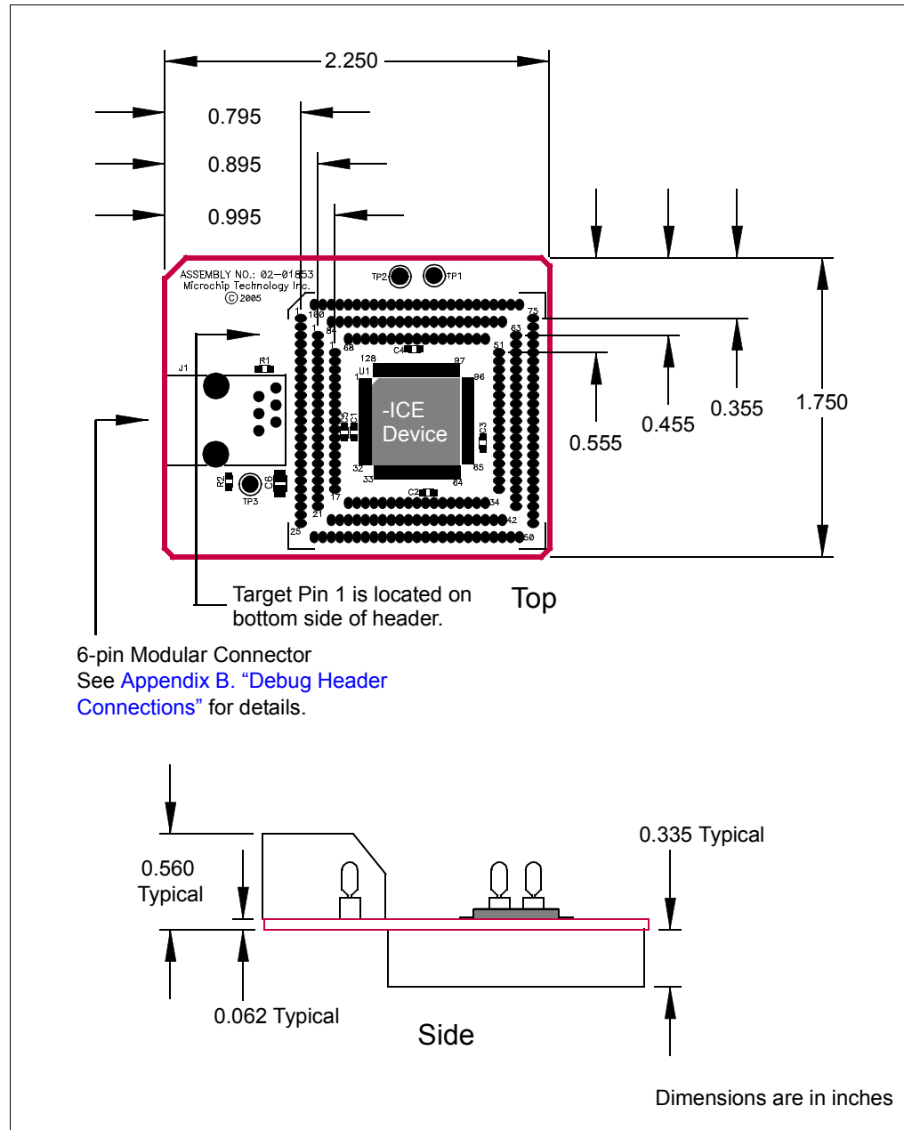
FIGURE 3-3: DIMENSIONS – AC162064
