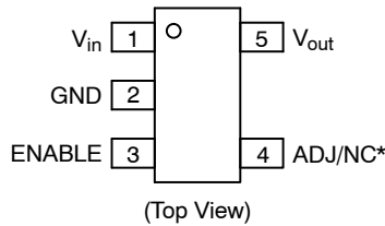
Figure 2. TSOP5
