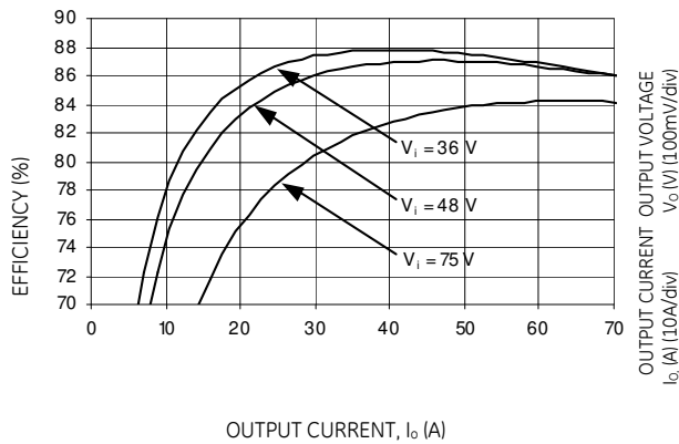
Figure 32. Converter Efficiency Vs Load at Room temperature.
