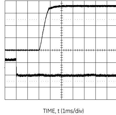
Figure 28. Typical Start-Up Characteristics from Remote ON/OFF.
