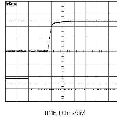
Figure 40. Typical Start-Up Characteristics from Remote ON/OFF.
