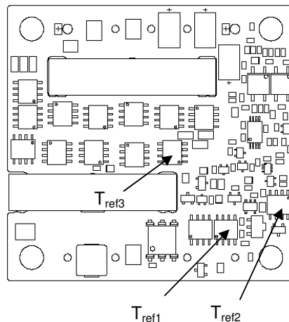
Figure 52. T_{ref} Temperature Measurement Locations for V_o=3.3V - 1.2V .
