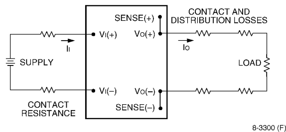
Figure 44. Output Ripple and Noise Test Setup.
