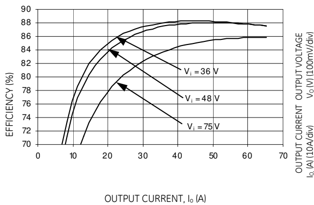
Figure 26. Converter Efficiency Vs Load at Room temperature.
