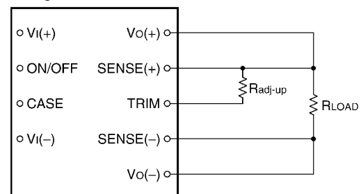
Figure 49. Circuit Configuration to Increase Output Voltage.
