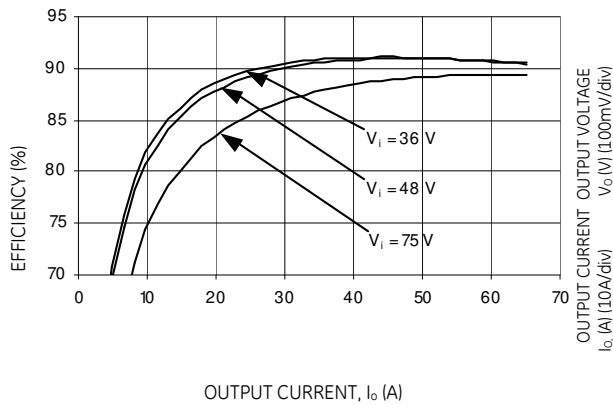
Figure 20. Converter Efficiency Vs Load at Room temperature.
