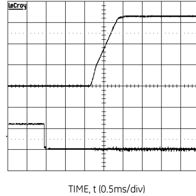
Figure 16. Typical Start-Up Characteristics from Remote ON/OFF.
