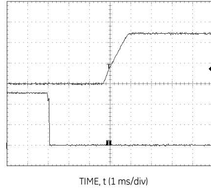
Figure 10. Typical Start-Up Characteristics from Remote ON/OFF.
