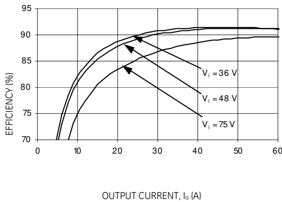
Figure 14. Converter Efficiency Vs Load at Room temperature.
