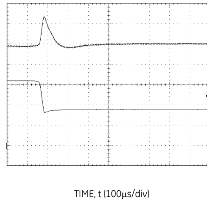
Figure 23. Transient Response to Dynamic Load Change from 50% to 25% of full load current.
