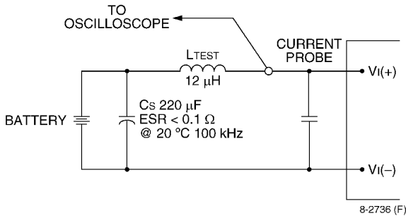
Figure 43. Input Reflected Ripple Current Test Setup.
