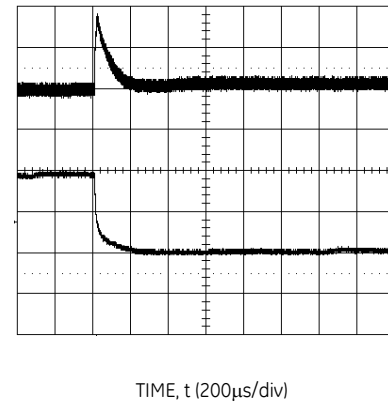
Figure 35. Transient Response to Dynamic Load Change from 50% to 25% of full load current.
