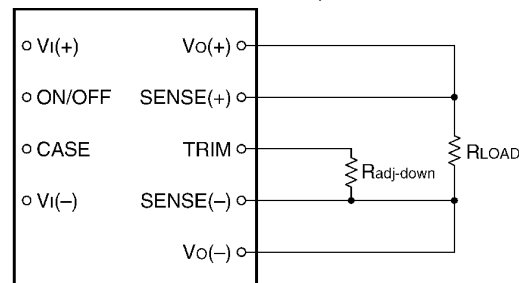
Figure 48. Circuit Configuration to Decrease Output Voltage.
