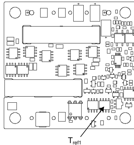
Figure 51. T_{ref} Temperature Measurement Location for V_o=5V .
