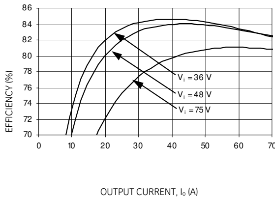
Figure 38. Converter Efficiency Vs Load at Room temperature.
