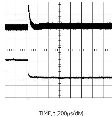
Figure 29. Transient Response to Dynamic Load Change from 50% to 25% of full load current.
