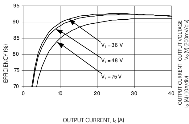
Figure 8. Converter Efficiency Vs Load at Room temperature.
