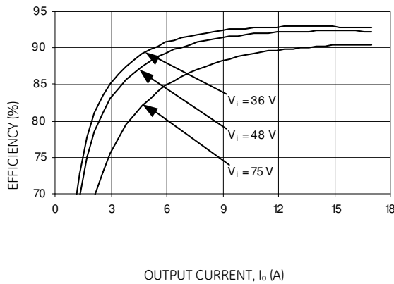
Figure 2. Converter Efficiency Vs Load at Room temperature.
