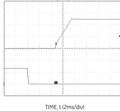
Figure 22. Typical Start-Up Characteristics from Remote ON/OFF.
