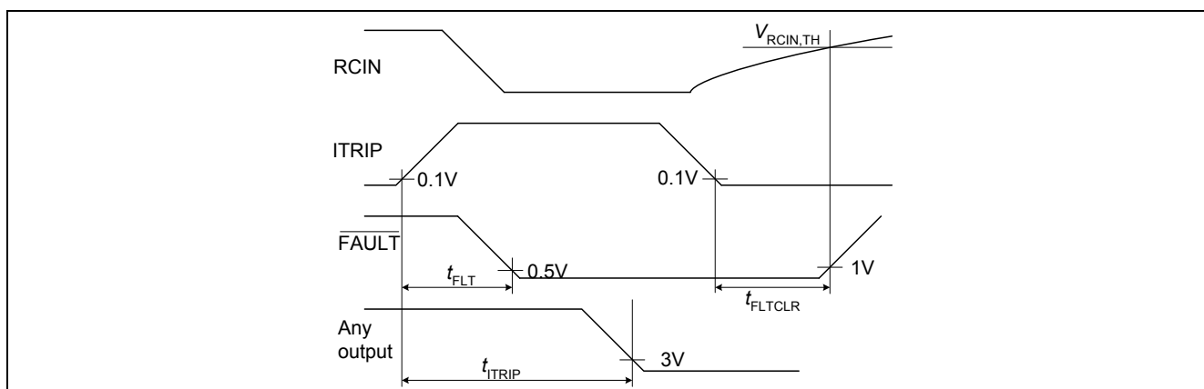
Figure 13 ITRIP-Timing
