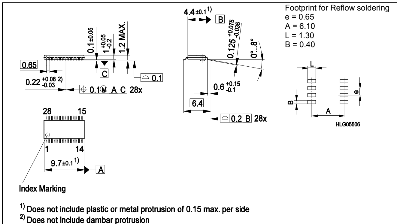
Figure 16 Package drawing
