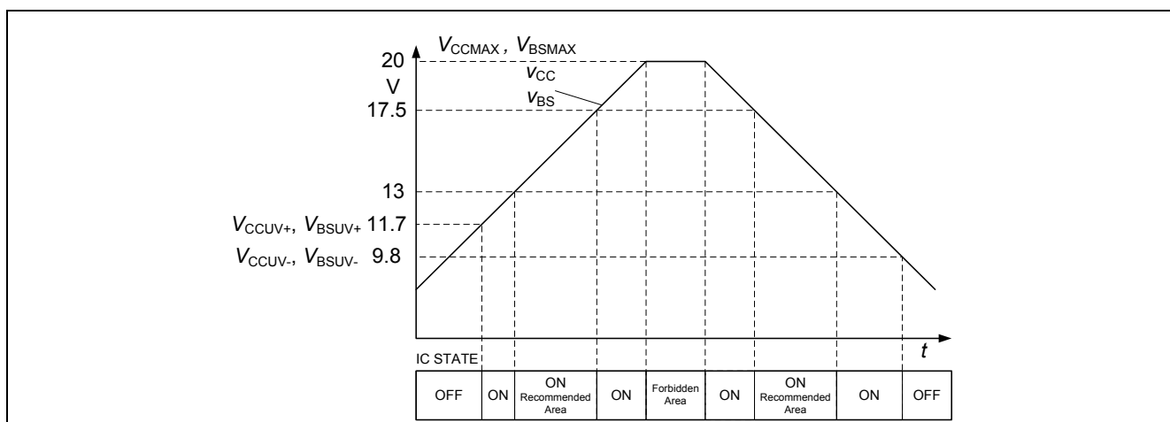
Figure 12 Operating areas
