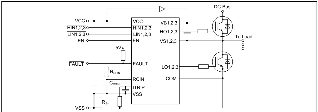
Figure 1 Typical Application
