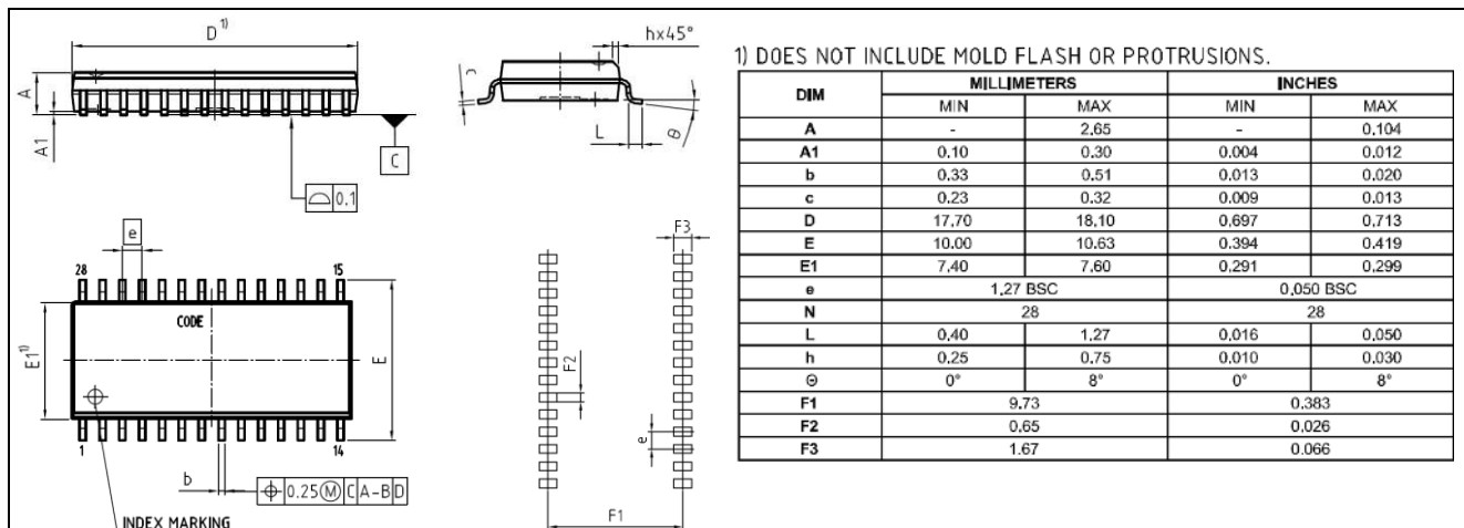
Figure 14 Package drawing
