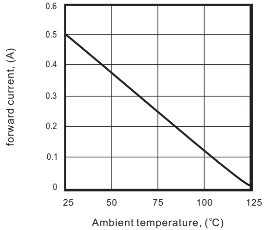
Fig.4 - Power derating
