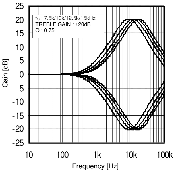
Figure 11. Treble fo vs Frequency
