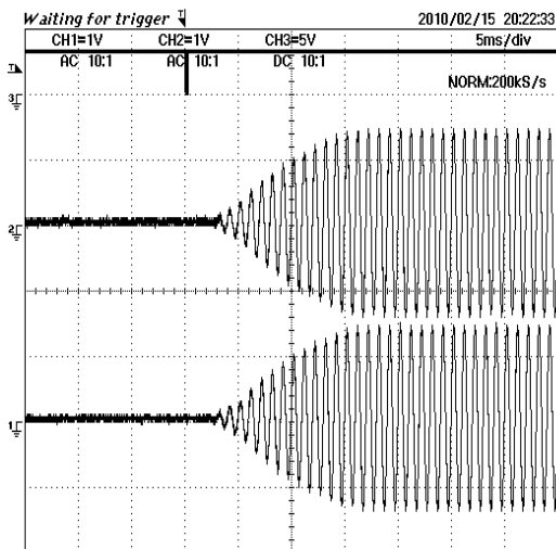
Figure 19. Advanced Switch 1
