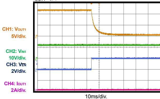
Shutdown through Enable (12V Efuse) I_{OUT1}=0A
