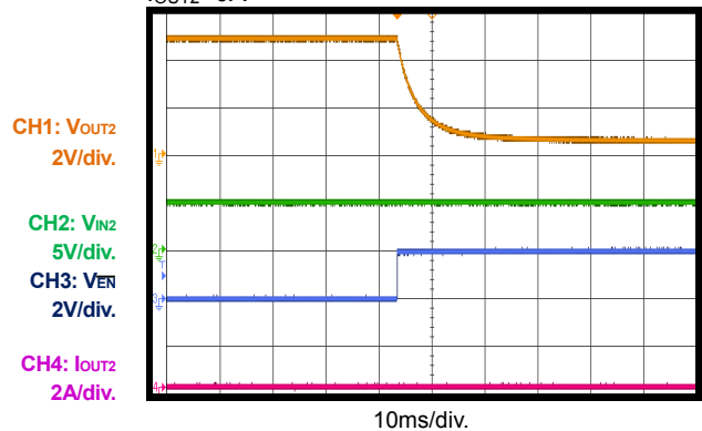
Shutdown through Enable (5V Efuse) I_{OUT2}=0A
