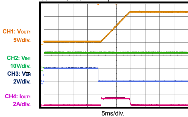
Start-Up through Enable (12V Efuse) I_{OUT1}=0A , C_{OUT1}=1000\mu\text{F}
