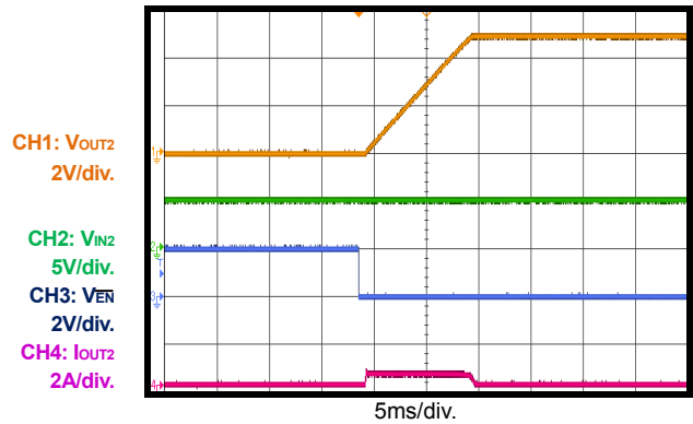
Start-Up through Enable (5V Efuse) I_{OUT2}=0A , C_{OUT2}=1000\mu\text{F}
