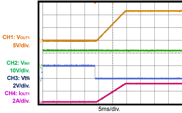
Start-Up through Enable (12V Efuse) I_{OUT1}=3A
