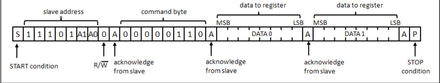
Figure 7: Write to configuration registers
