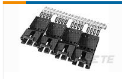
TE Part #5-103946-5 2X6 MTE SHRD PIN SR POL .100CL
