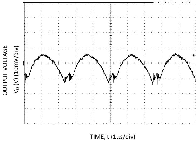
Figure 9. Typical output ripple and noise (C 0 = 6x47µF ceramic, V IN = 12V, I o = I o,max ).
