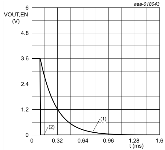
V_{I(VIN)} = 3.6\text{ V}; R_L = 10\ \Omega; C_L = 20\ \mu\text{F}; T_{amb} = 25\ ^\circ\text{C} (1) VOUT (2) EN
