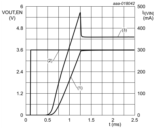
V_{I(VIN)} = 3.6\text{ V}; R_L = 10\ \Omega; C_L = 20\ \mu\text{F}; T_{amb} = 25\ ^\circ\text{C}. (1) VOUT (2) EN (3) I_{I(VIN)}
