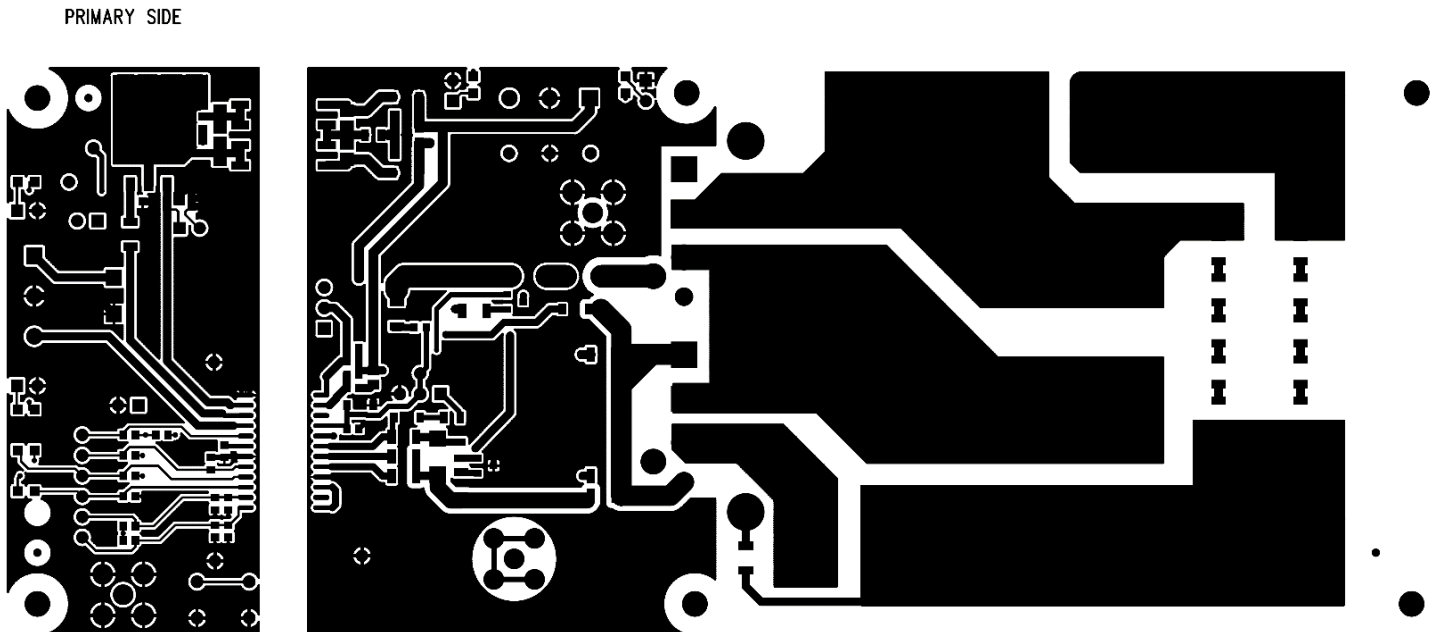
Figure 5.2. Si8284v2-EVB Top Copper
