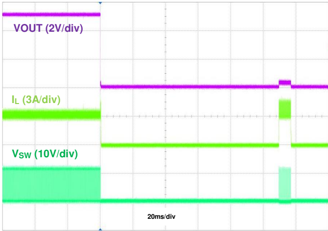
Figure 35. Output Short Protection, IOOUT = 3A
