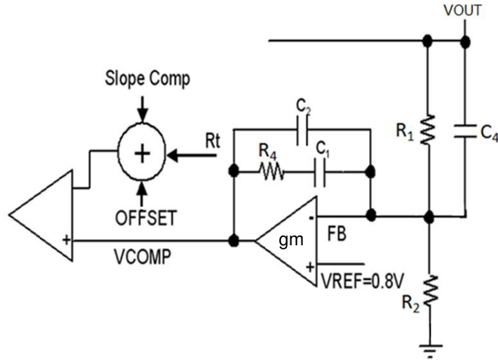
Figure 46. Type 2 Compensator
