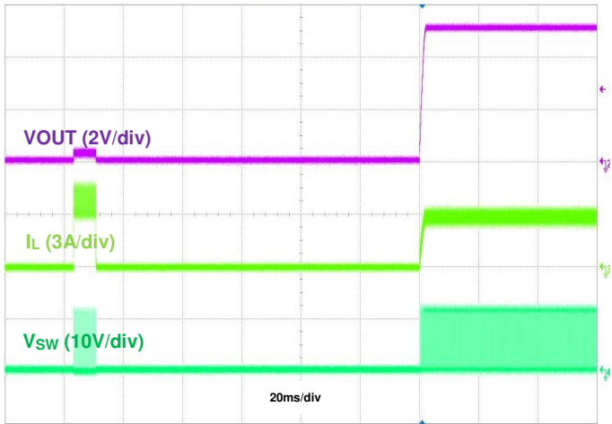
Figure 36. Output Short Recovery, IOOUT = 3A
