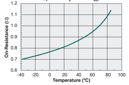
Typical On-Resistance vs. Temperature ( I_F=2\text{mA} , I_L=600\text{mA}_{DC} )
