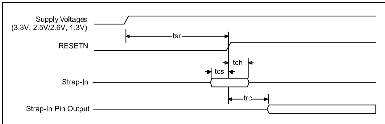
FIGURE 5-1: RESET TIMING
