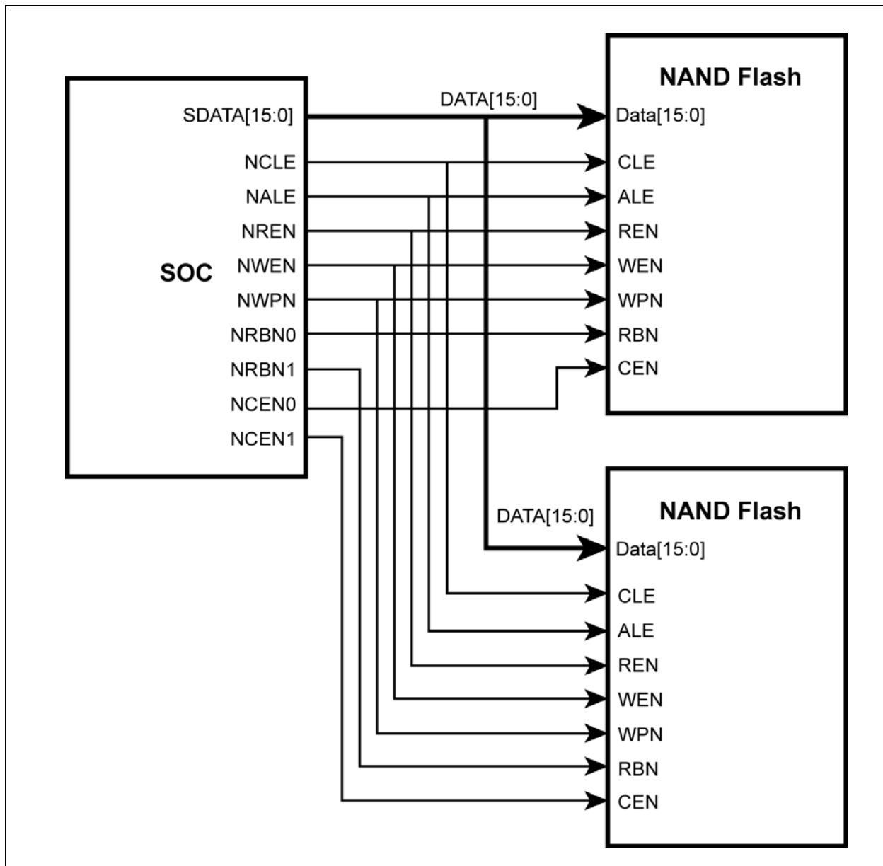
FIGURE 2-6: 16-BIT NAND INTERFACE EXAMPLES
