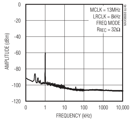
WIDEBAND FFT, 0dBFS (DAC TO RECEIVER)
