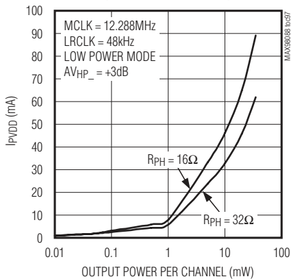
PVDD CURRENT vs. OUTPUT POWER (DAC TO HEADPHONE)
