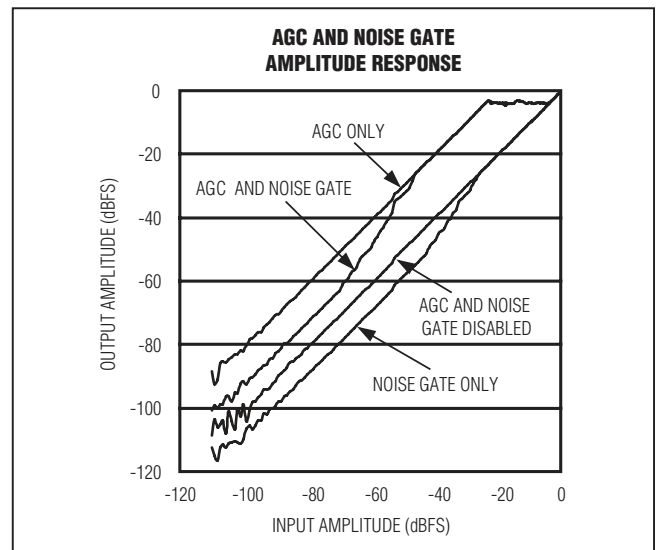
Figure 11. AGC and Noise Gate Input vs. Output Gain
