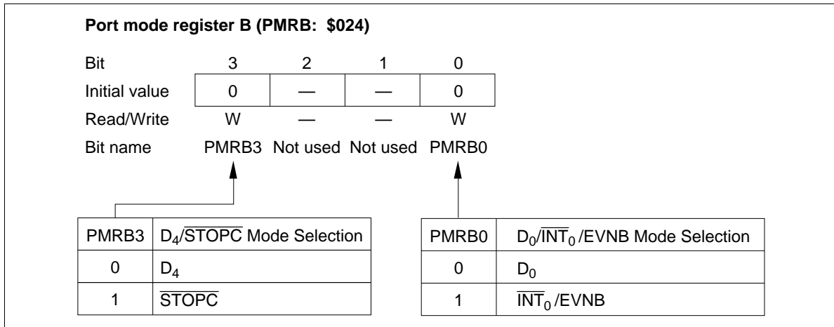
Figure 20 Port Mode Register B (PMRB)
