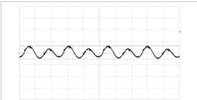
Output voltage ripple at: T_{P1} = +25^\circ\text{C} , V_I = 53\text{ V} , I_O = 32.5\text{ A} resistive load.
