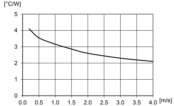
Thermal resistance vs. airspeed measured at the converter. Tested in wind tunnel with airflow and test conditions as per the Thermal consideration section. V_I = 53 V.
