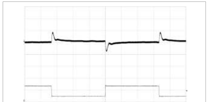
Output voltage response to load current step- change (8.1 – 24.4 – 8.1 A) at: T_{P1} = +25^\circ\text{C} , V_I = 53\text{ V} .
