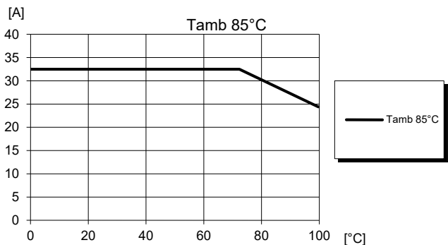
Available load current vs. cold wall temperature. V_I = 53 V. See Thermal Consideration section.
