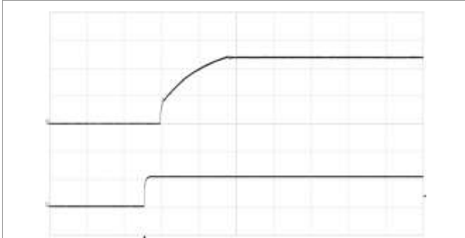
Start-up enabled by connecting V_I at: T_{P1} = +25^\circ\text{C} , V_I = 53\text{ V} , I_O = 32.5\text{ A} resistive load.
