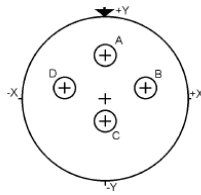
Contact Layout
