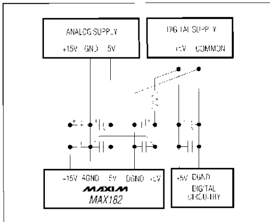
Figure 16 Power-Supply Grounding
