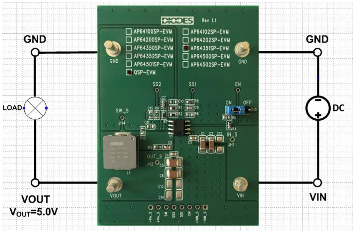
Figure 2. AP64351QSP-EVM
