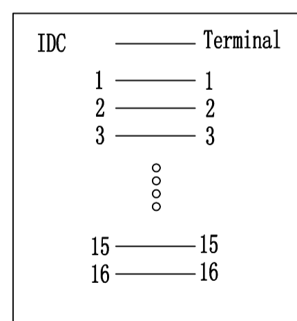
Pin assignment
