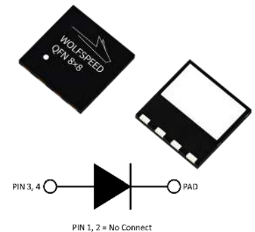
Package Types: QFN 8x8 Marking: C6D06065Q
