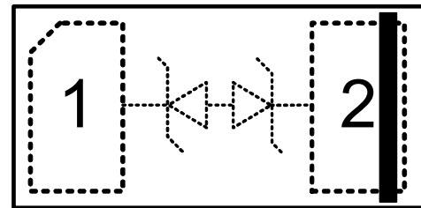
DFN1.0x0.6_2L (Top View)
