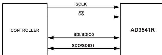
Figure 90. Dual SPI Connection
