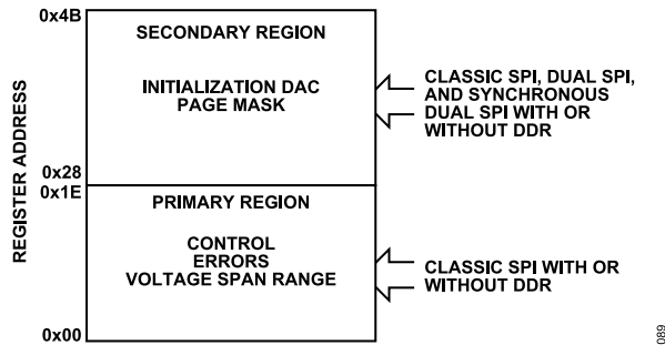
Figure 92. Register Access Modes
