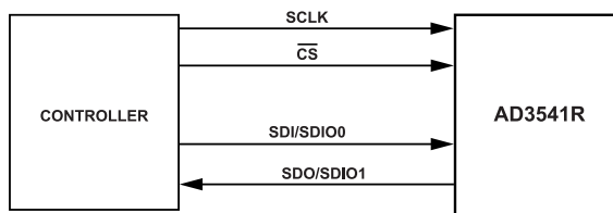
Figure 89. Single SPI (Classic SPI) Connection
