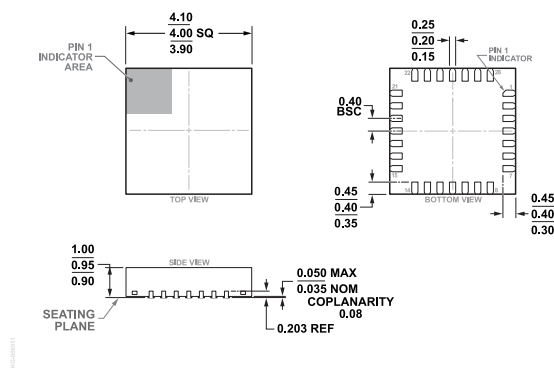
Figure 98. 28-Lead Lead Frame Chip Package [LFCSP] 4 mm x 4 mm Body and 0.95 mm Package Height (CP-28-15) Dimensions shown in millimeters
