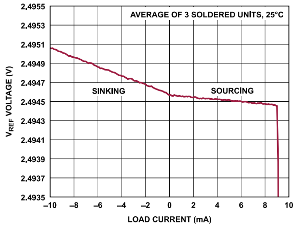
Figure 65. V REF Voltage vs. Load Current
