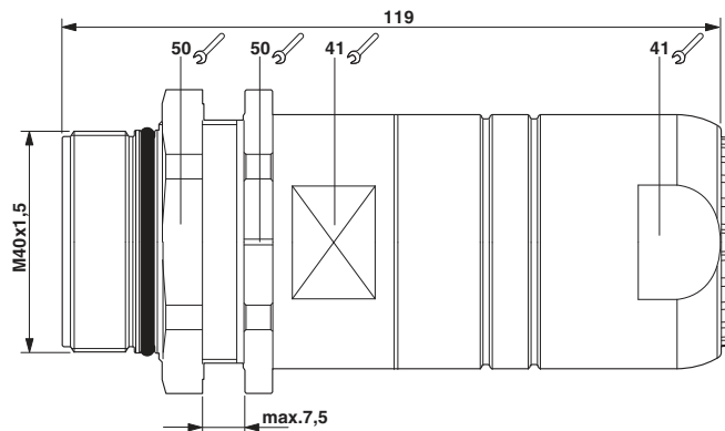
Dimensioned drawing
