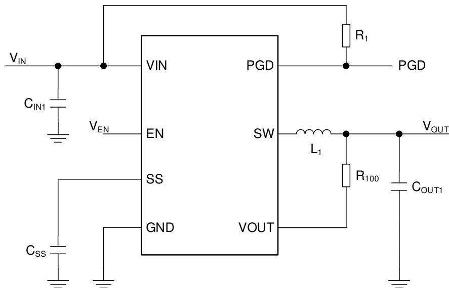
Figure 27. Typical Application
