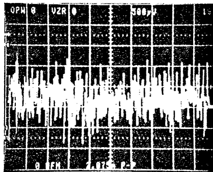
0.1Hz TO 1MHz NOISE V_{CC} = \pm 15V, T_A = +25^\circ C 500μV/Div., 1s/Div., A_V = 1000 V/V Total Output Noise = 2.075μVp-p
