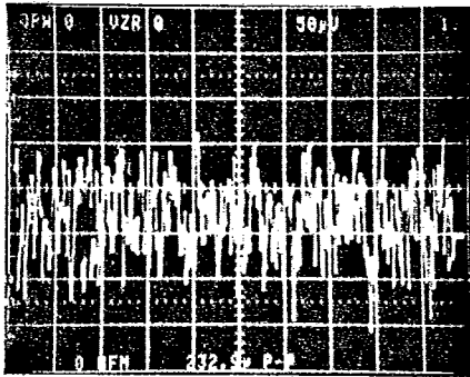
0.1Hz TO 10Hz NOISE V_{CC} = \pm 15V, T_A = +25^\circ C 50μV/Div., 1s/Div., A_V = 1000 V/V Input Noise = 0.232μVp-p
