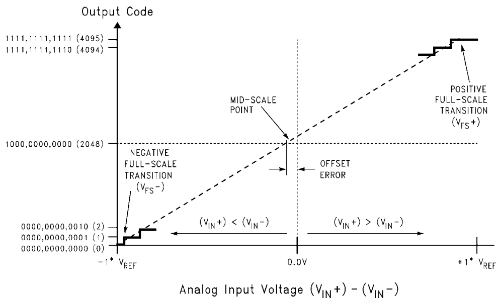
FIGURE 1. Transfer Characteristic (Offset Binary Format)
